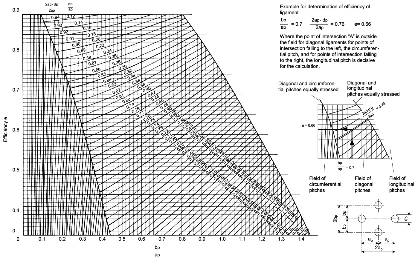
Figure 8 Ligament efficiencies — staggered drilling
