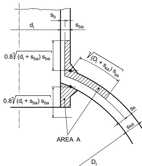
b) Reinforcement area, K = 0.7
