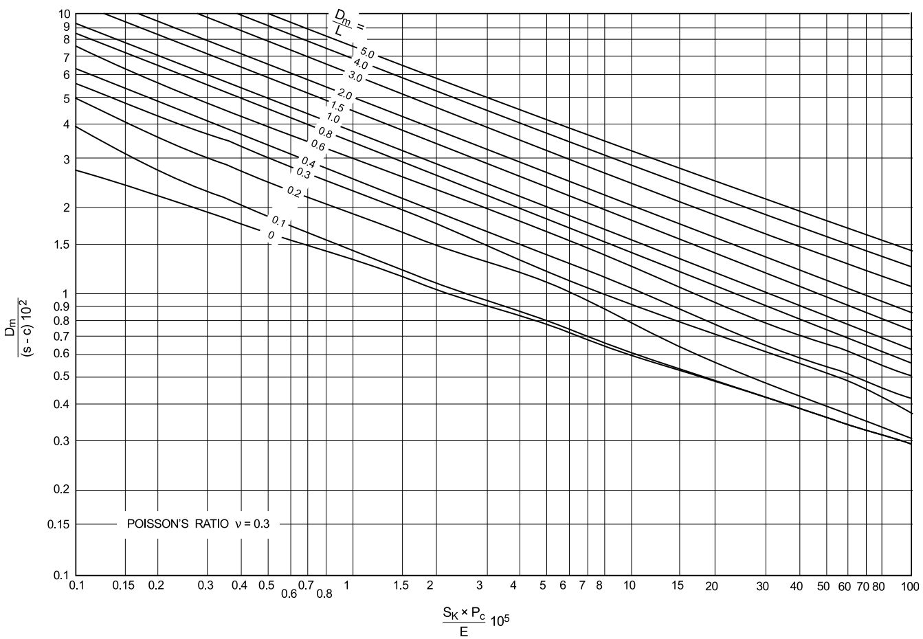
Figure 29 Required thickness by calculation against elastic instability
