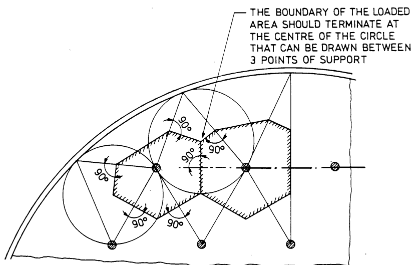
Figure 33 Loaded area on stays
