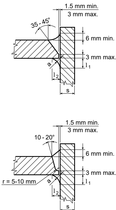
Figure 15 Attachment of un-flanged flat end plates or tube plates to shell (examples)
