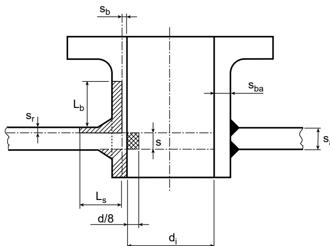
Figure 28 Compensation of openings in flat plates
