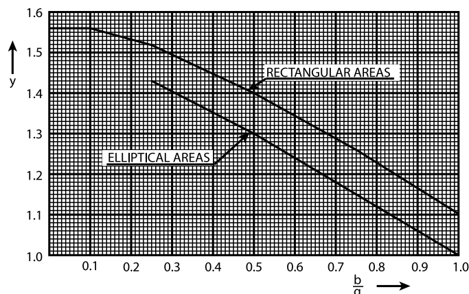
Figure 19 Determination of factor y
