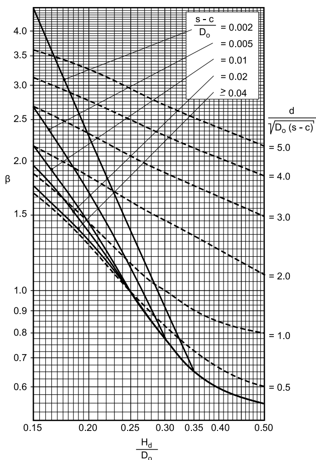
Figure 13 Graph of shape factor \beta for dished ends
