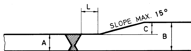
CIRCUMFERENTIAL JOINTS WHERE C EXCEEDS 10 % OF B + 1 mm OR 4 mm
