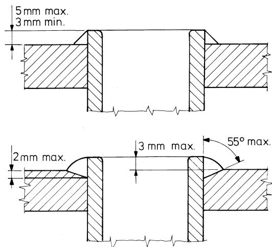
Figure 22 Typical attachment of welded plain tubes
