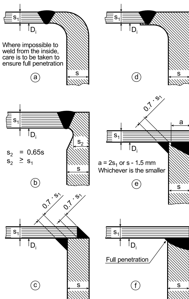
Figure 17 Acceptable methods of attaching flat end plates to cylindrical shells
