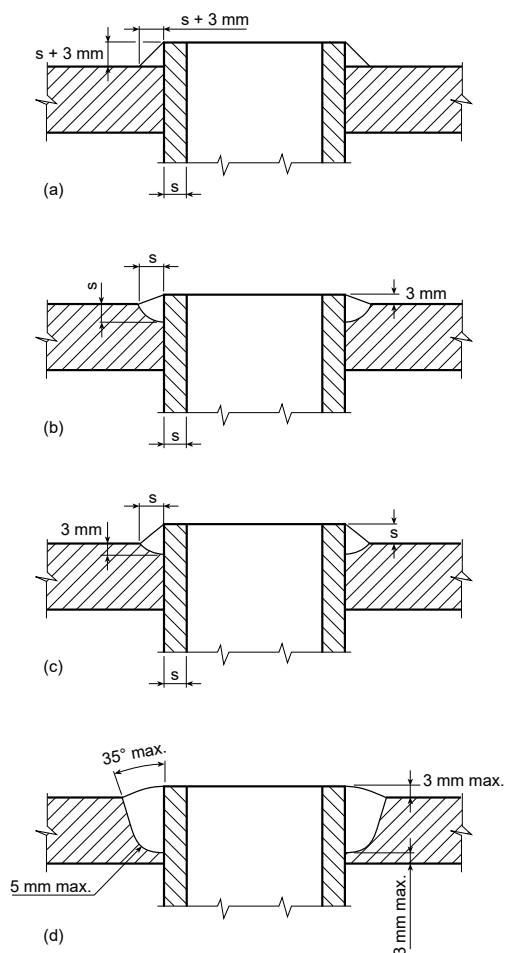
Figure 21 Typical attachment of stay tubes
