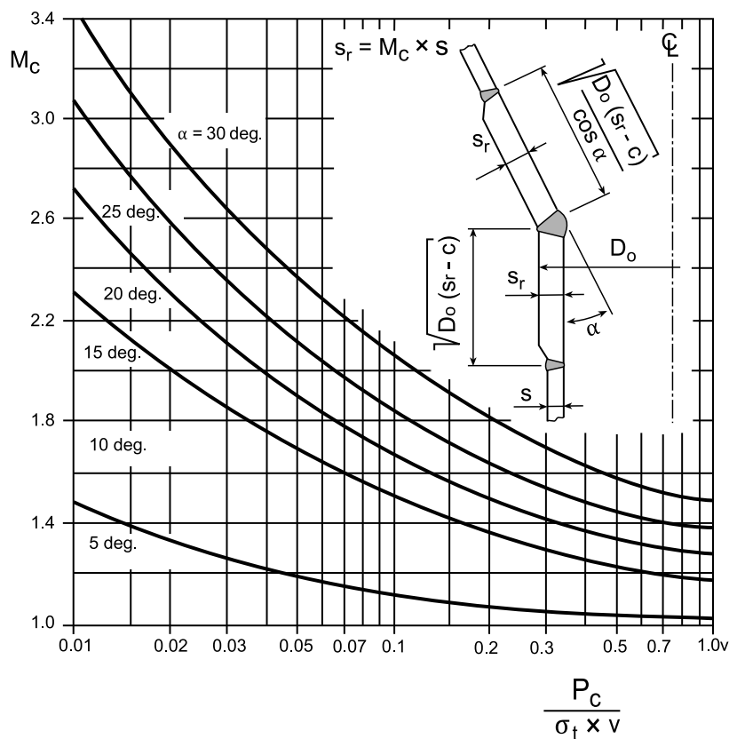
Figure 3 Values of M_C for small end cone-cylinder junction
