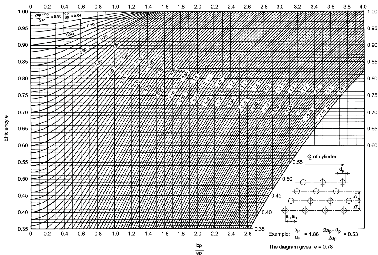
Figure 6 Ligament efficiencies — diagonal drilling
