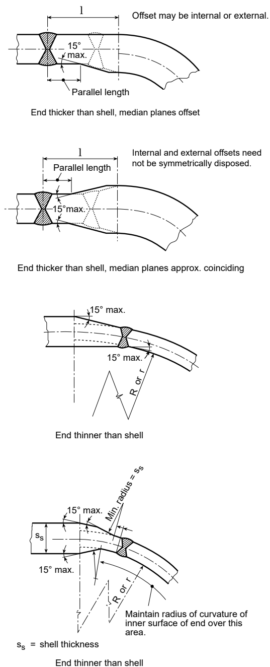
Figure 14 Dished ends — cylindrical shell connections
