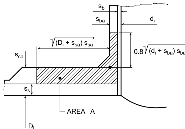
a) Reinforcement area, K=1
