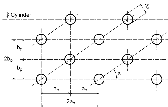
Figure 6 Ligament efficiencies — diagonal drilling
