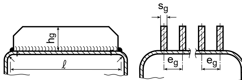
Figure 24 Unsupported girder
