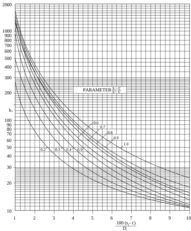
Figure 16 Calculation factor k_f
