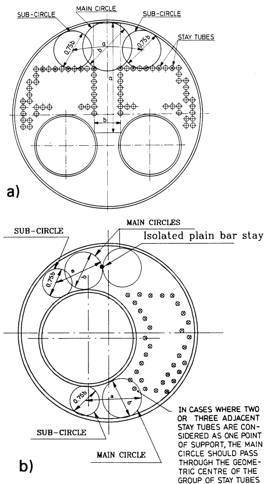
Figure 18 Use of sub-circles and rectangular areas
