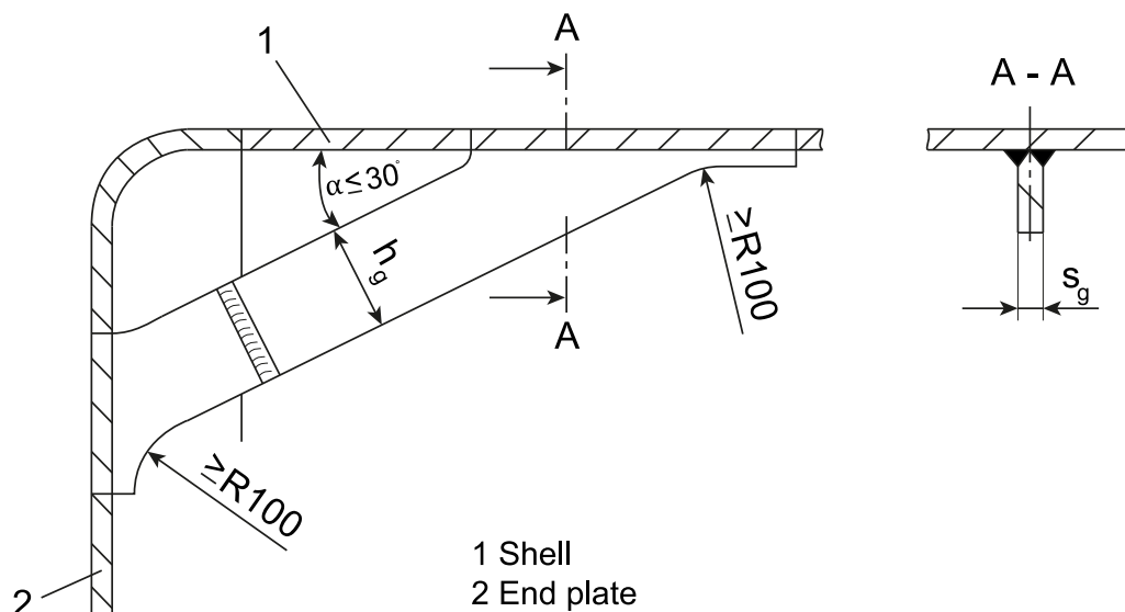
Figure 34 Details of welded gusset stays
